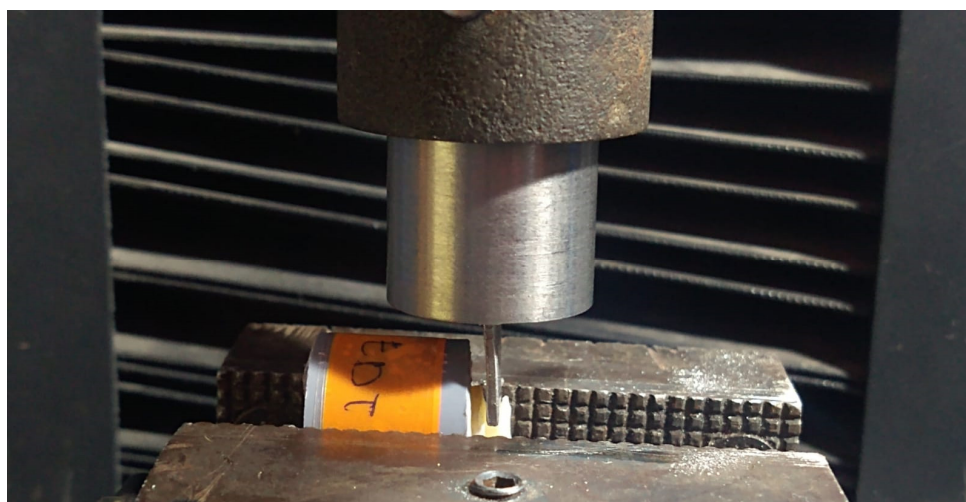
Figure 4. Shear test with universal testing machine.
